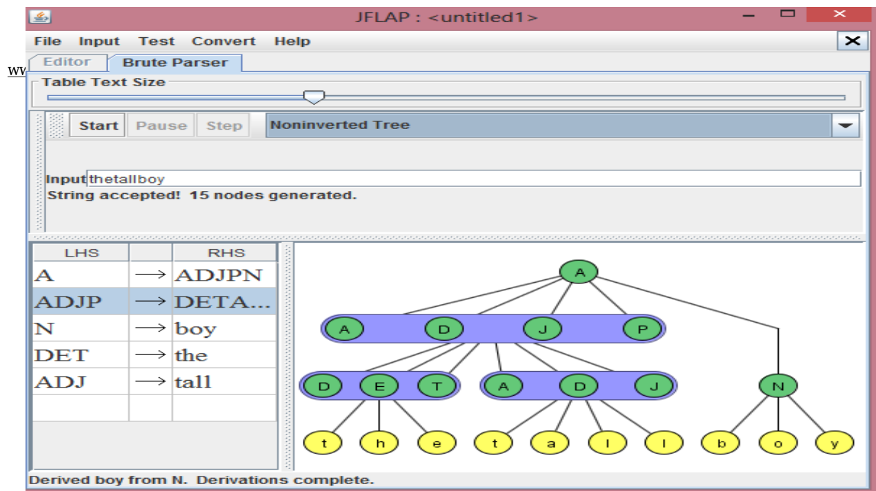
Figure 3: English Adjectival Phrase Rewrite Test
