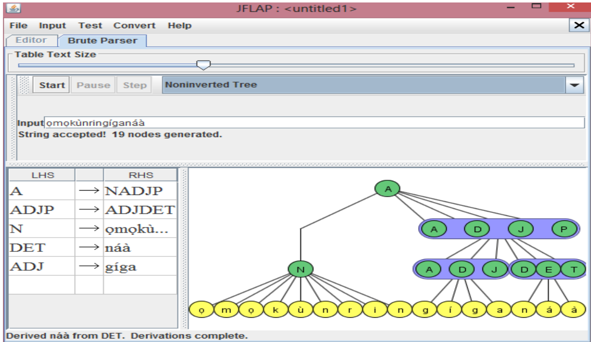
Figure 2: Yoruba Adjectival Phrase Rewrite Test
