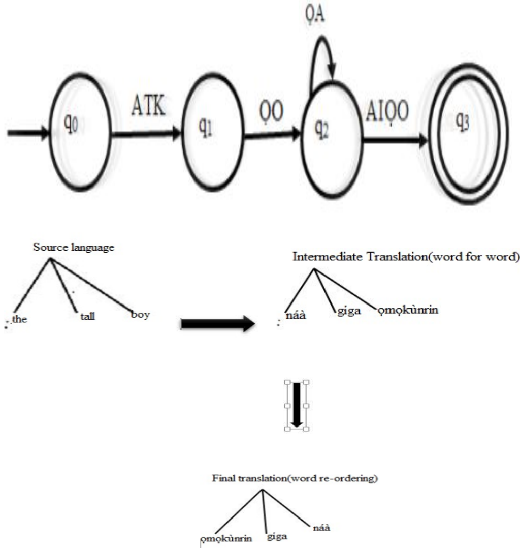
Figure 6: Adjectival Phrase Translation Process Abstraction
